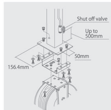
Installation example mm
