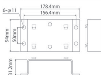
Mounting bracket dimensions mm
